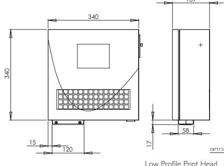
Low Profile Print Head
