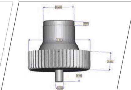
Check the dimensions of your parts
