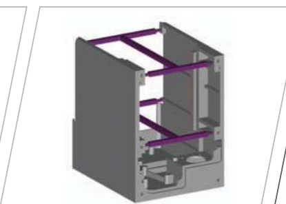
Avoid deformation by adding props
