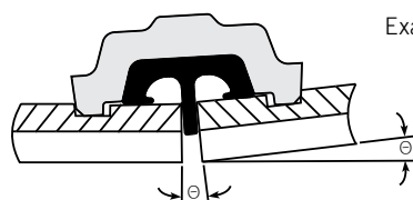
Deflection Angle at Each Coupling Listed in Degrees
