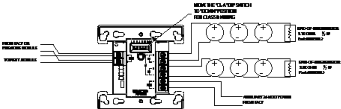
Typical Class A Wiring Diagram
