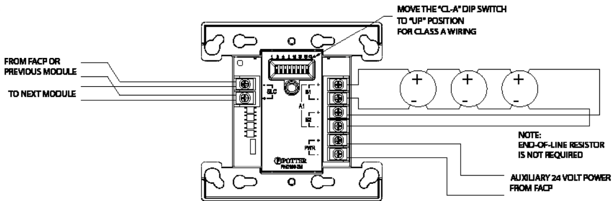
Typical Class A Wiring Diagram
